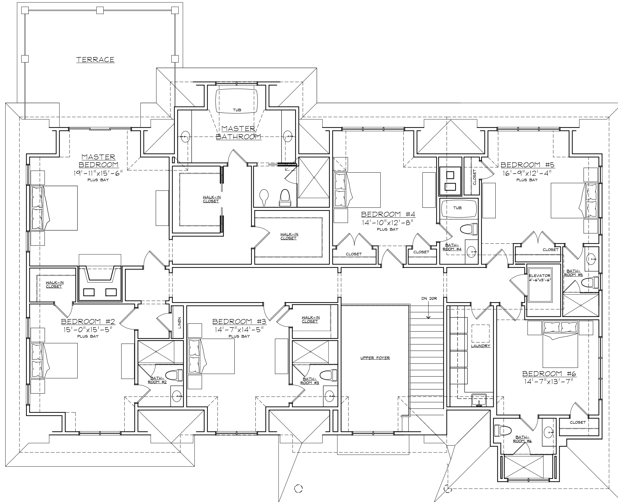
SECOND FLOOR PLAN 47 SOUTH HILL STREET
