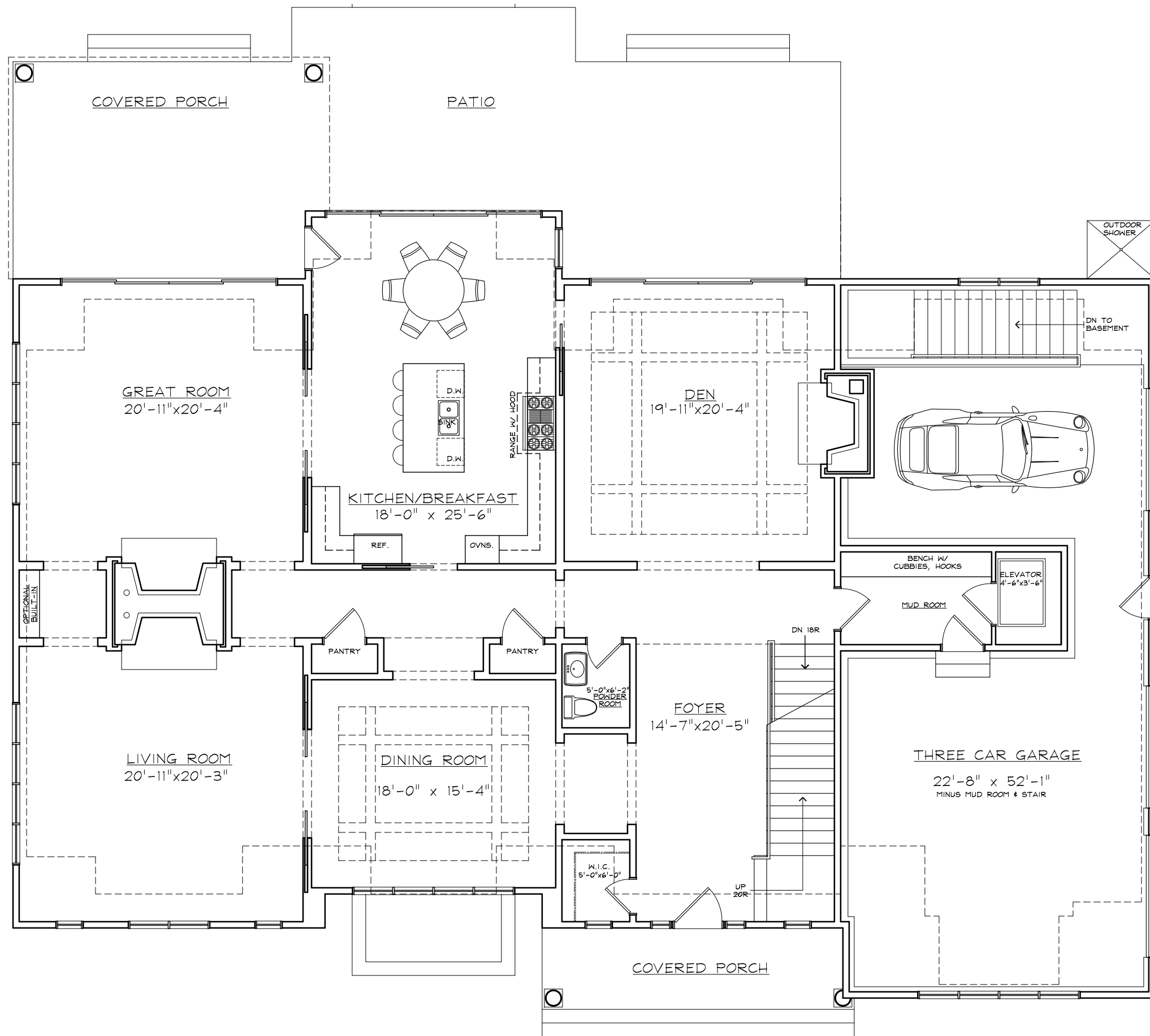
FIRST FLOOR PLAN 47 SOUTH HILL STREET
