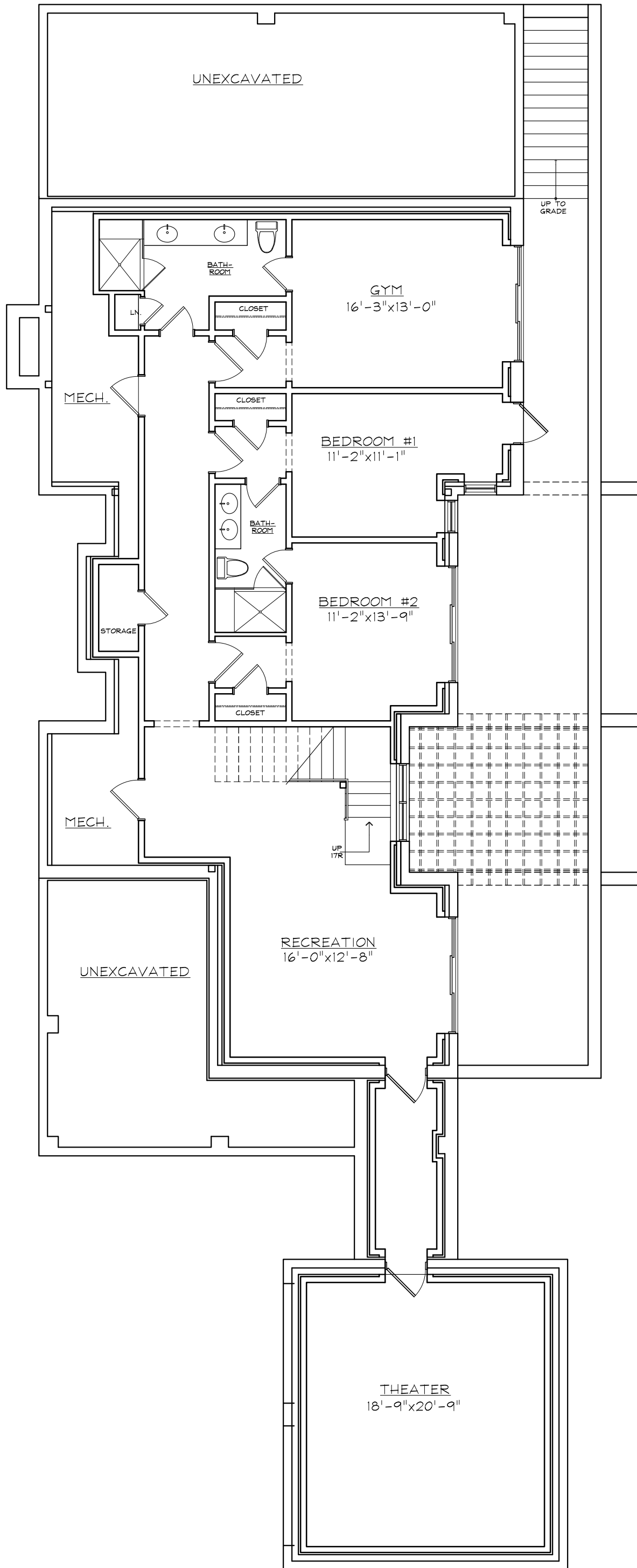
BASEMENT PLAN (12-16-13) MEETING HOUSE LANE
