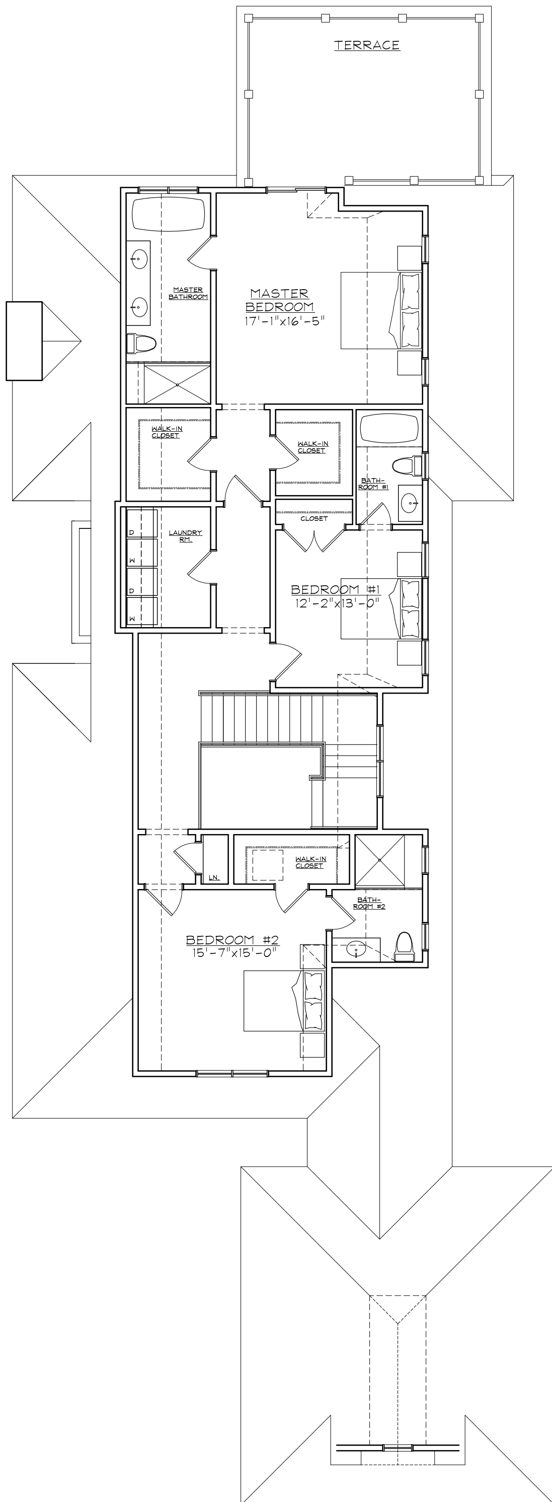
SECOND FLOOR PLAN (12-16-13) MEETING HOUSE LANE 1,547 SQ. FT.
