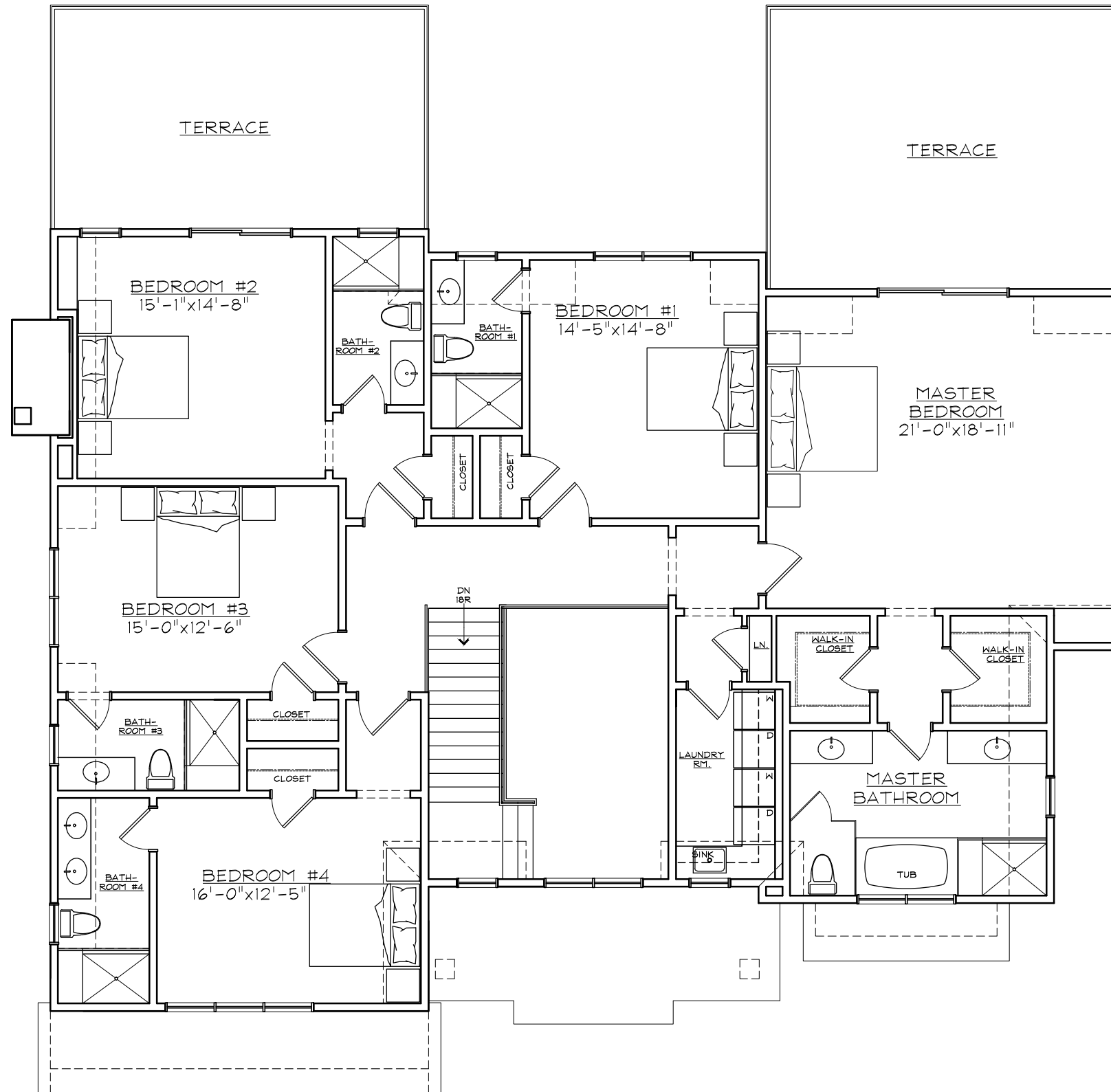
SECOND FLOOR PLAN DEERFIELD ROAD (LOT # 14) 2,366 SQ. FT.
