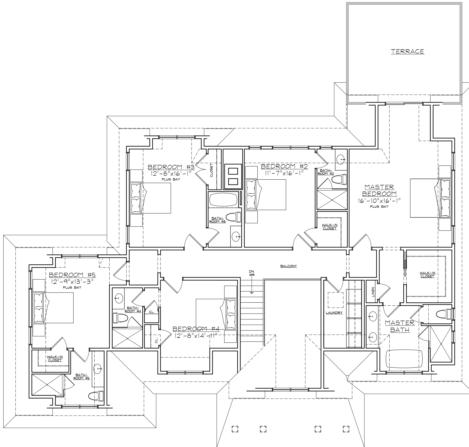
SECOND FLOOR PLAN DEERFIELD ROAD (LOT 16) 2,186 SQ. FT.
