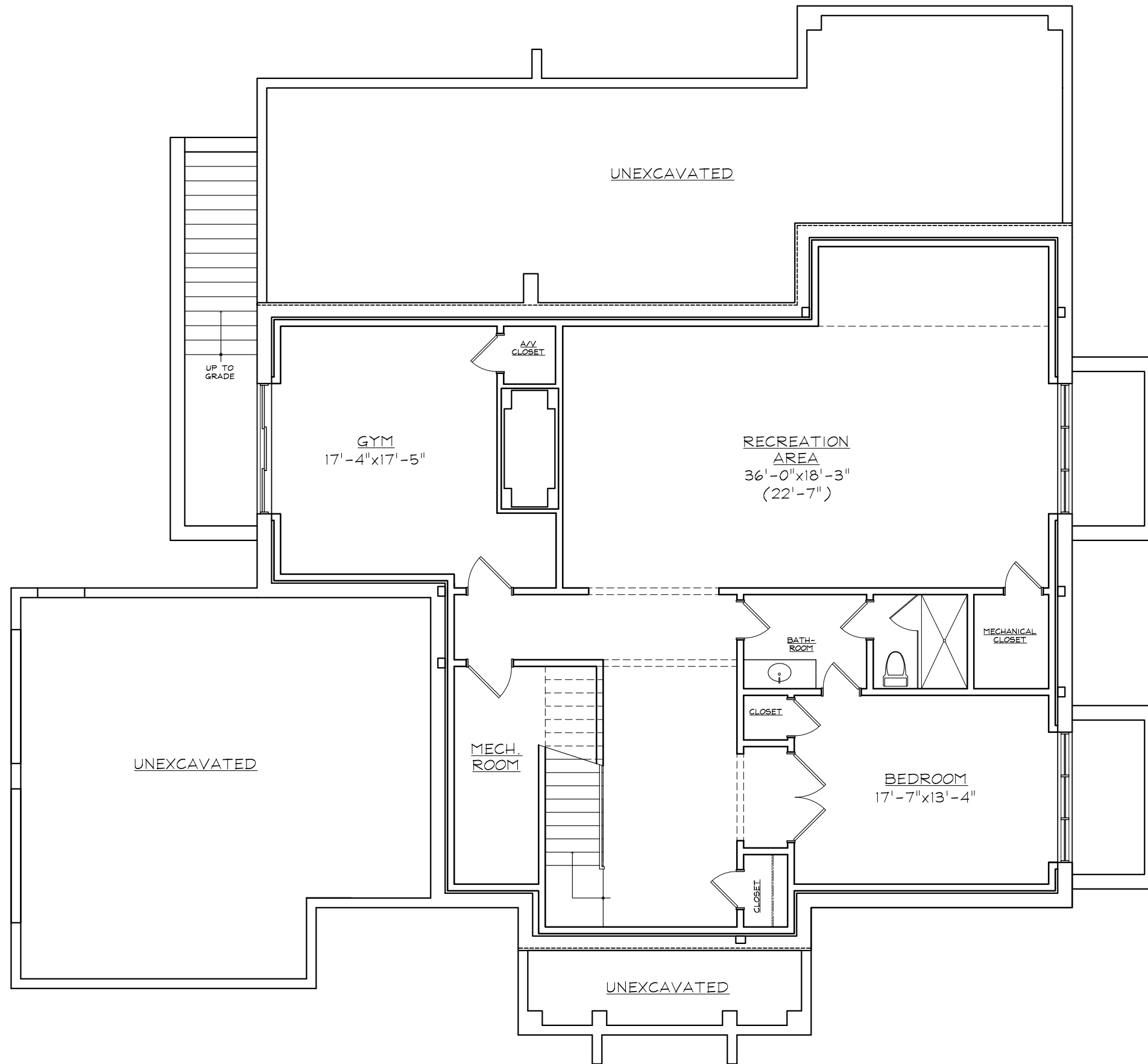
BASEMENT PLAN DEERFIELD ROAD (LOT 17) 1,904 SQ. FT.
