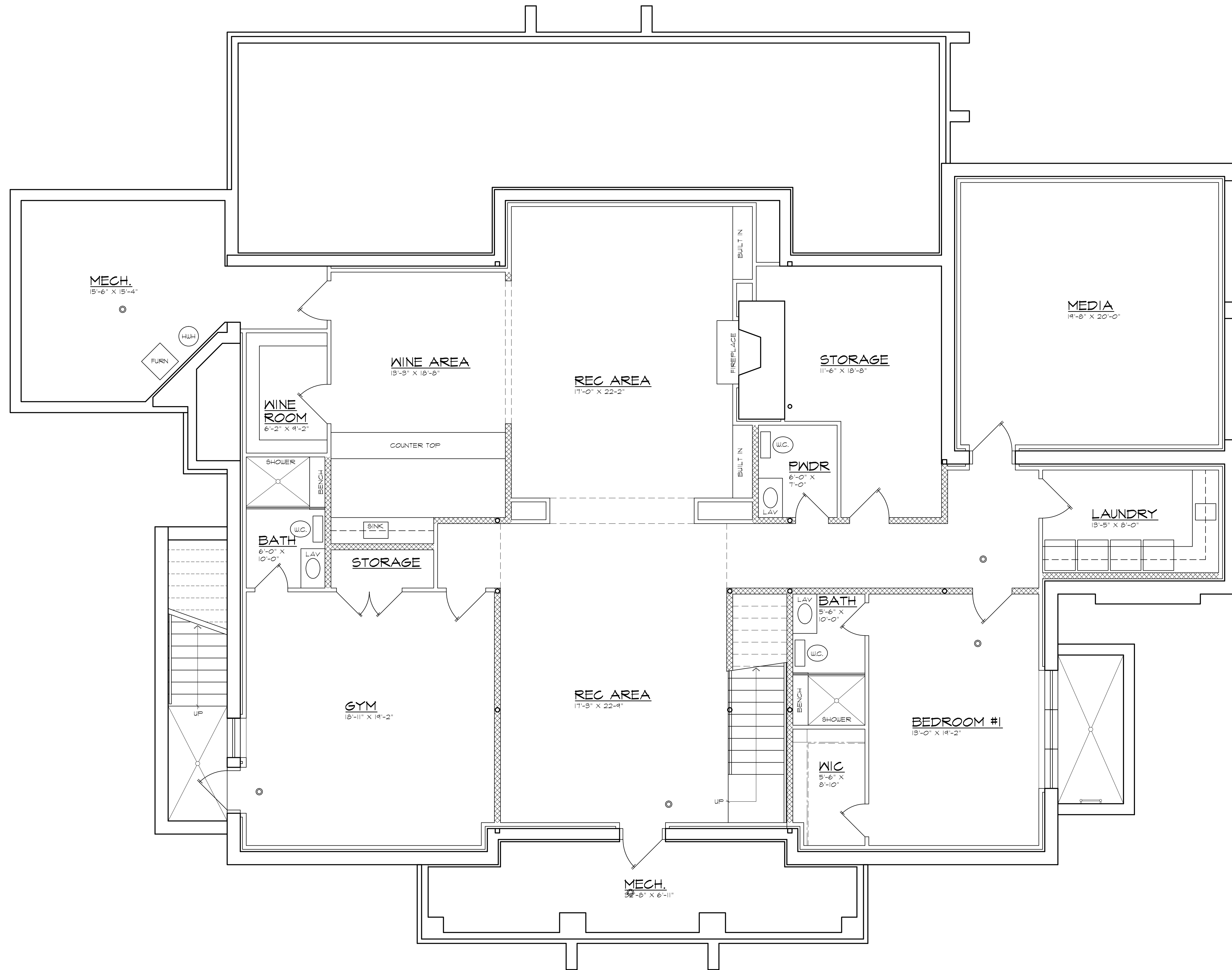
BASEMENT PLAN
