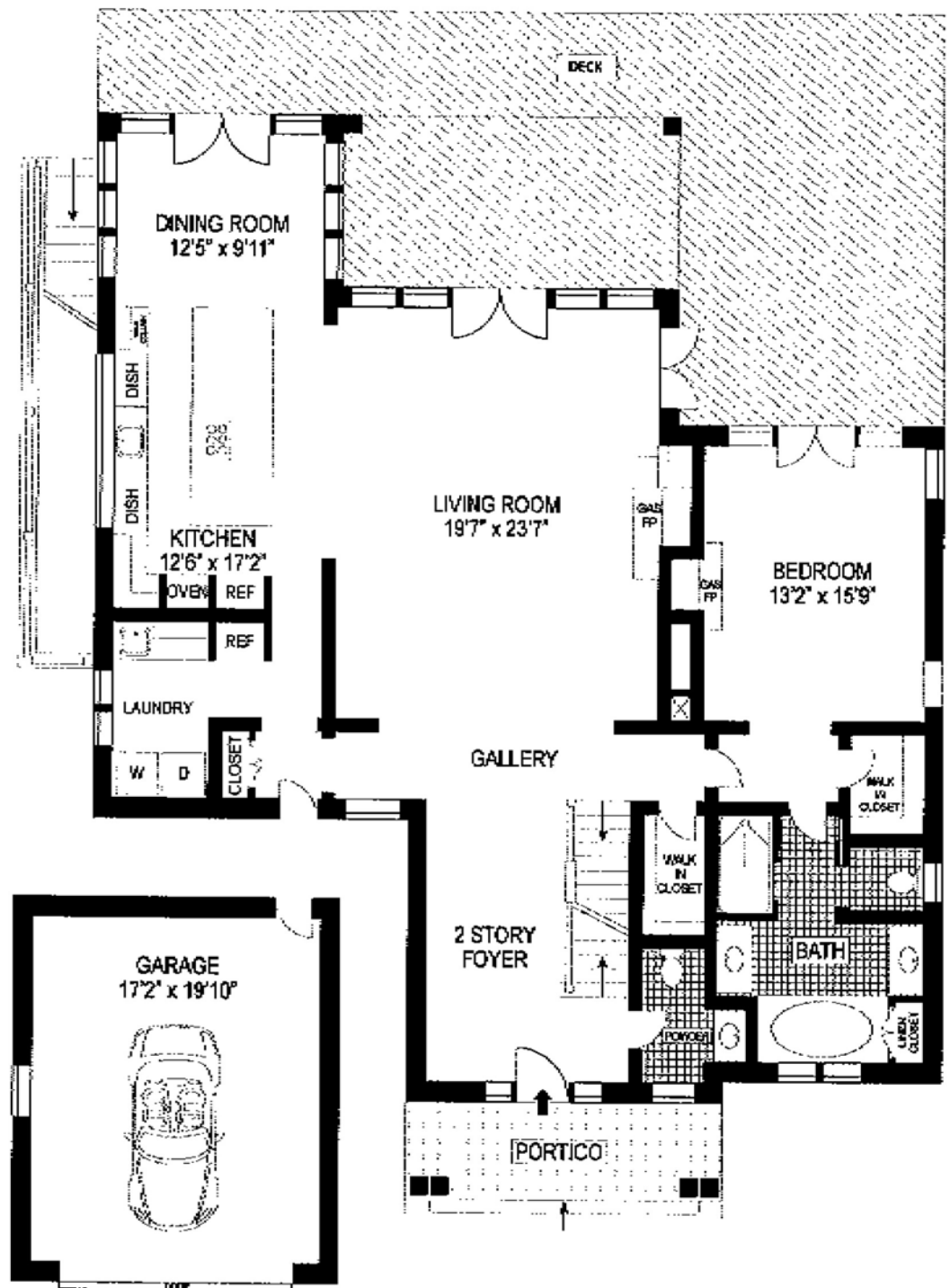
FIRST FLOOR
