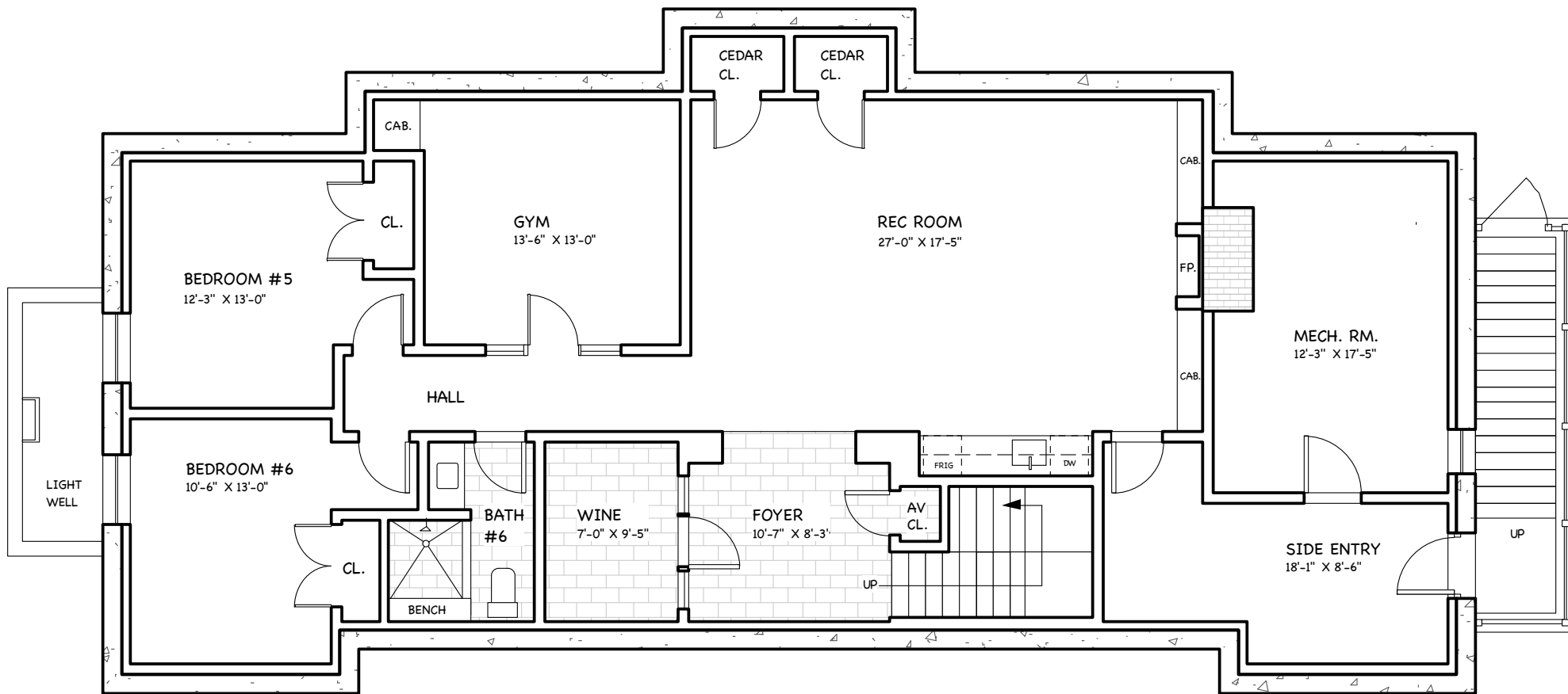
○ BASEMENT PLAN
