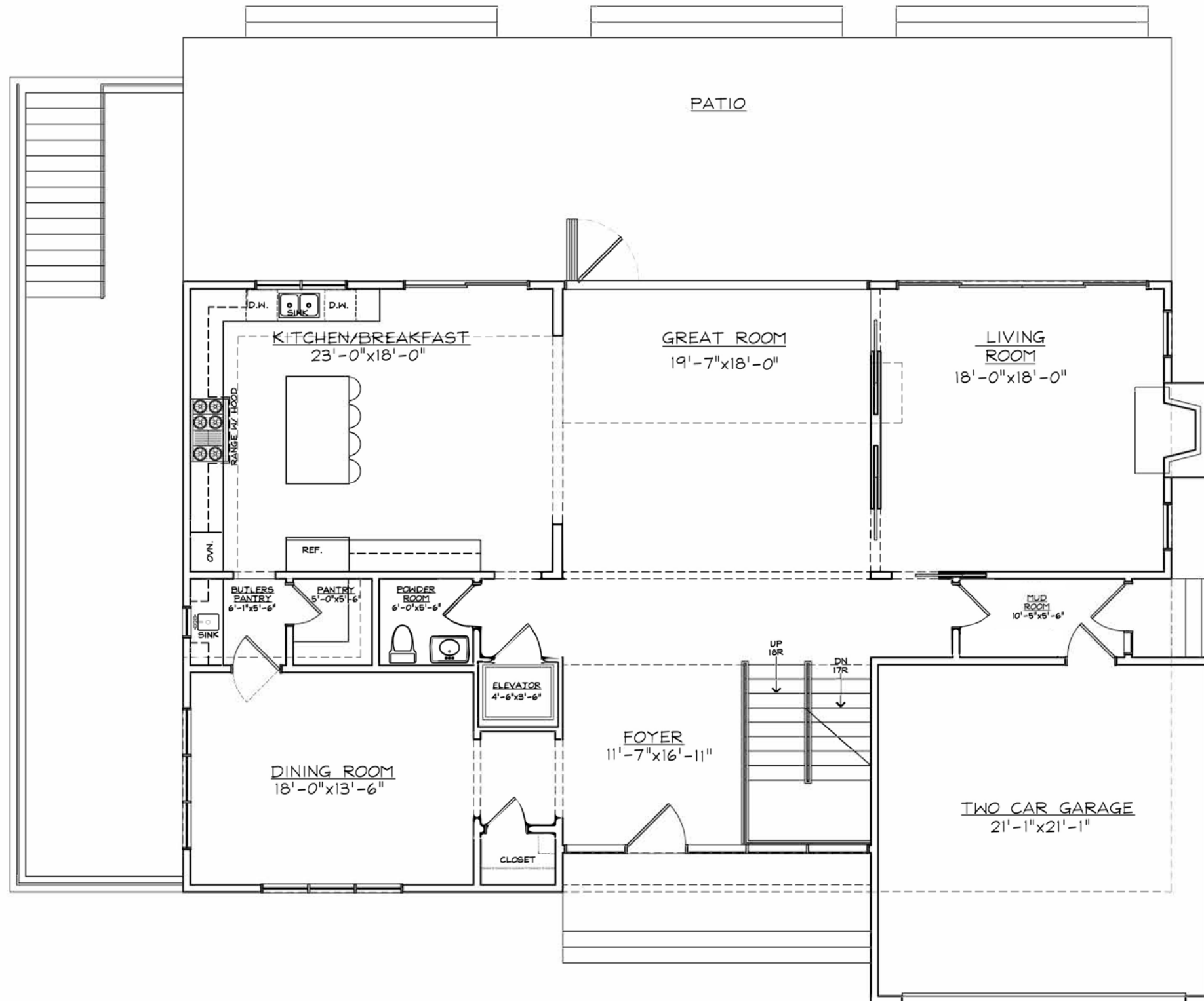
FIRST FLOOR PLAN (7-28-15)
