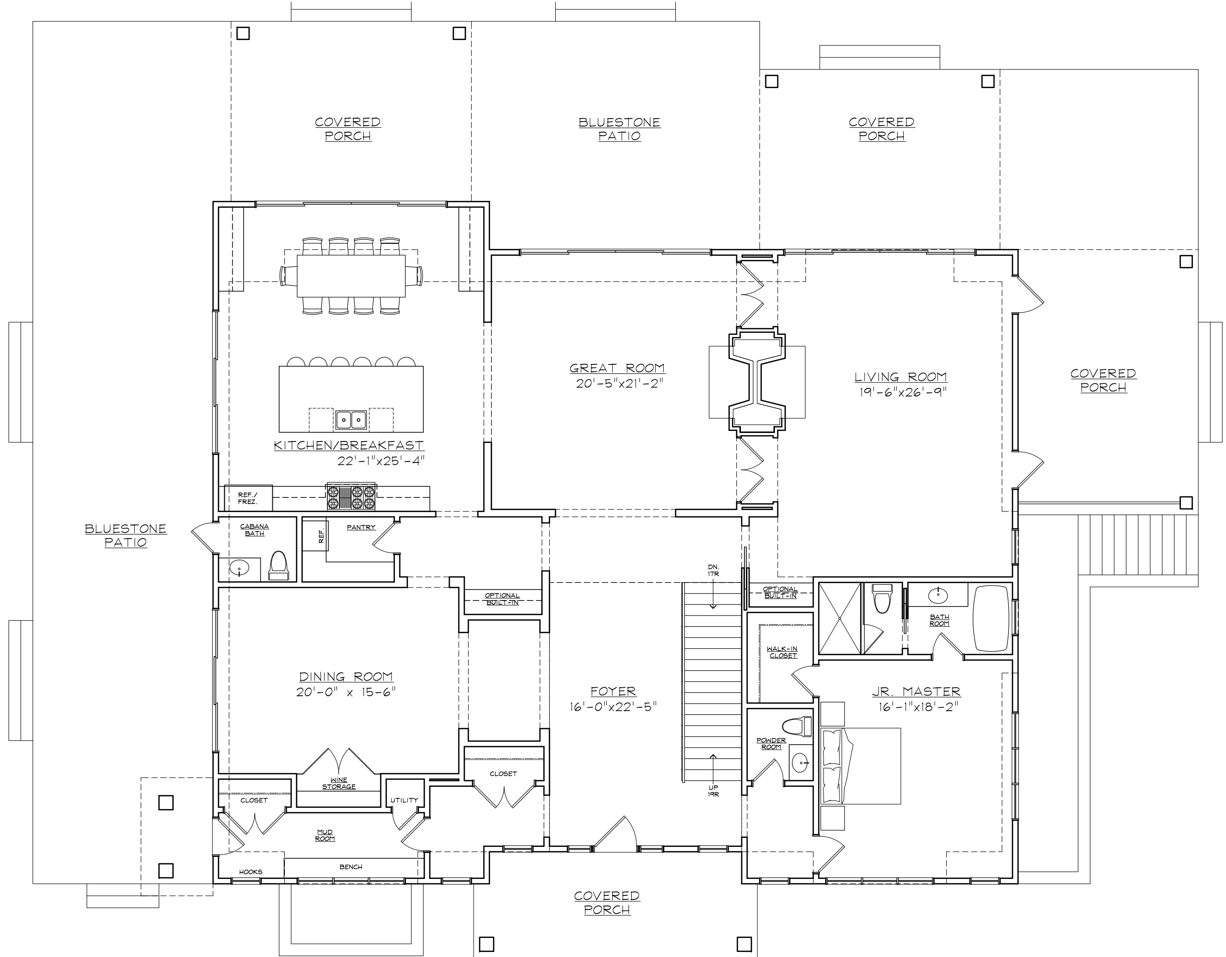
FIRST FLOOR PLAN DEERFIELD LOT 7
