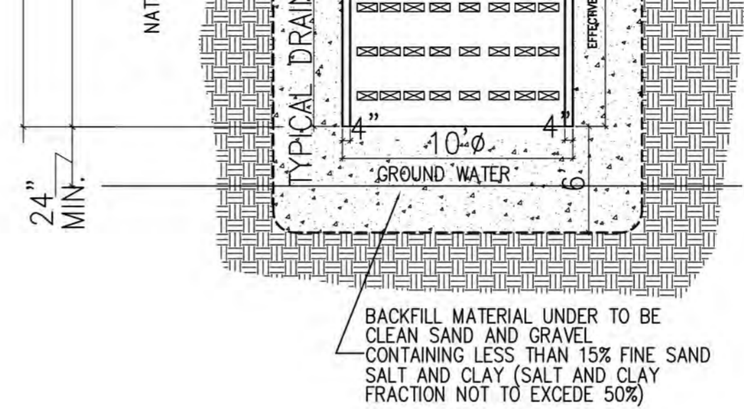
3 DRYWELL DETAIL SCALE: (NTS)
