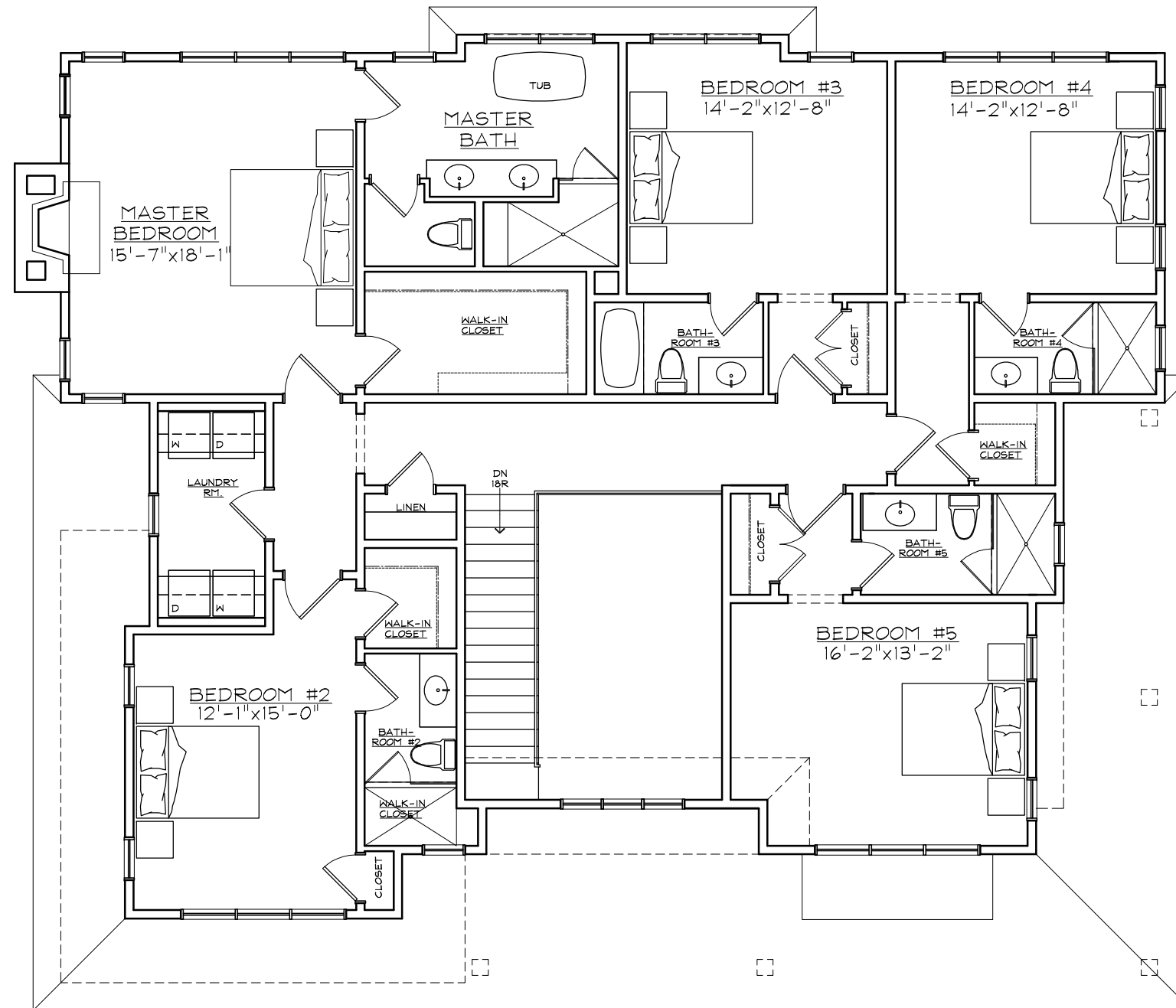
SECOND FLOOR PLAN RUGGS PATH (LOT 3)
