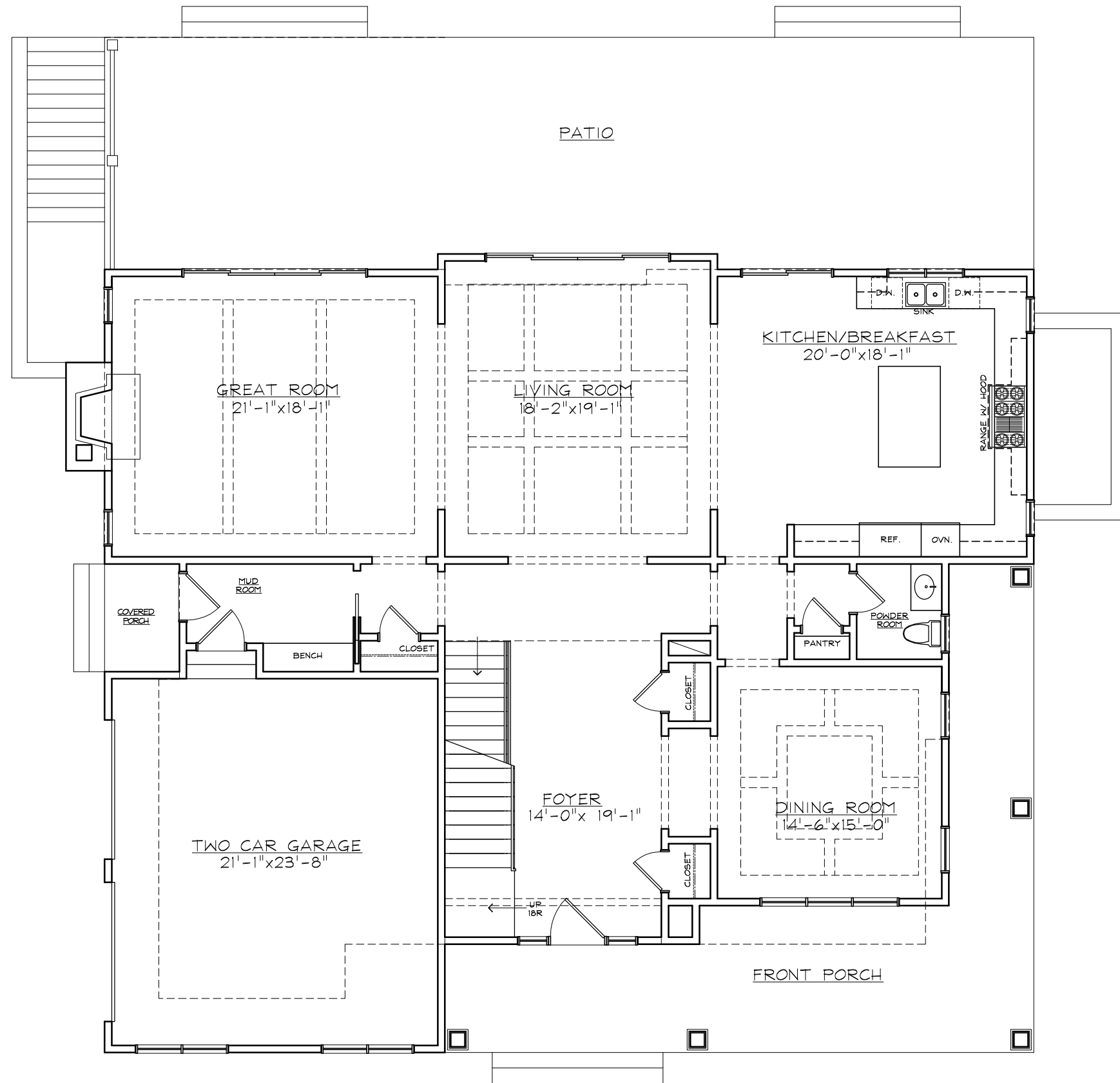
FIRST FLOOR PLAN RUGGS PATH (LOT 3)
