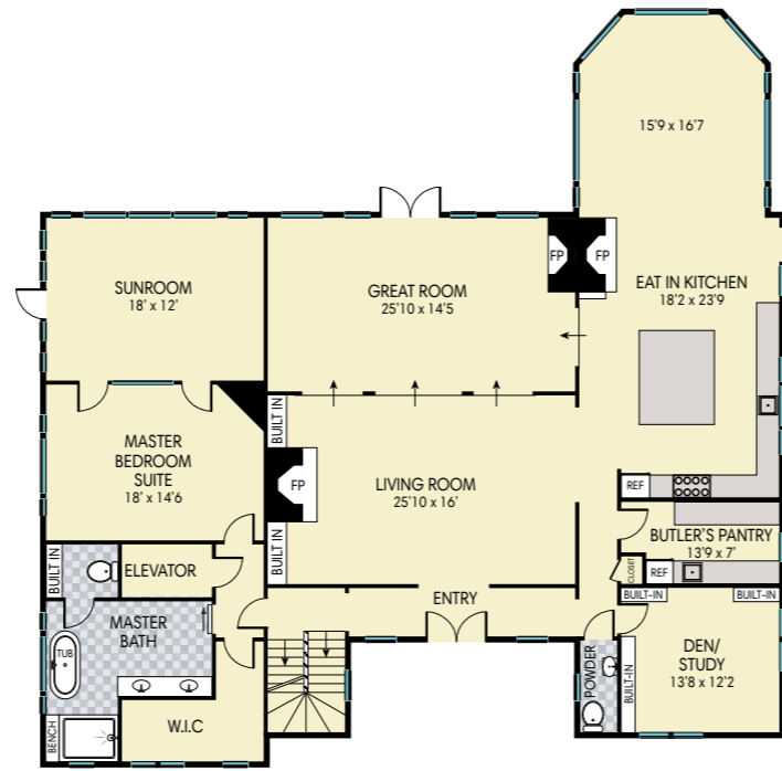
MAIN HOUSE - FIRST FLOOR
