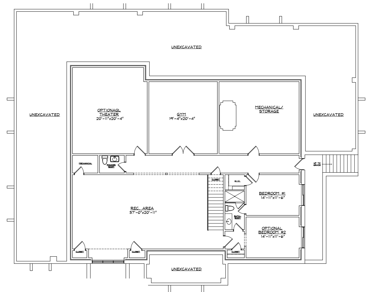
Lower Level Floorplan
