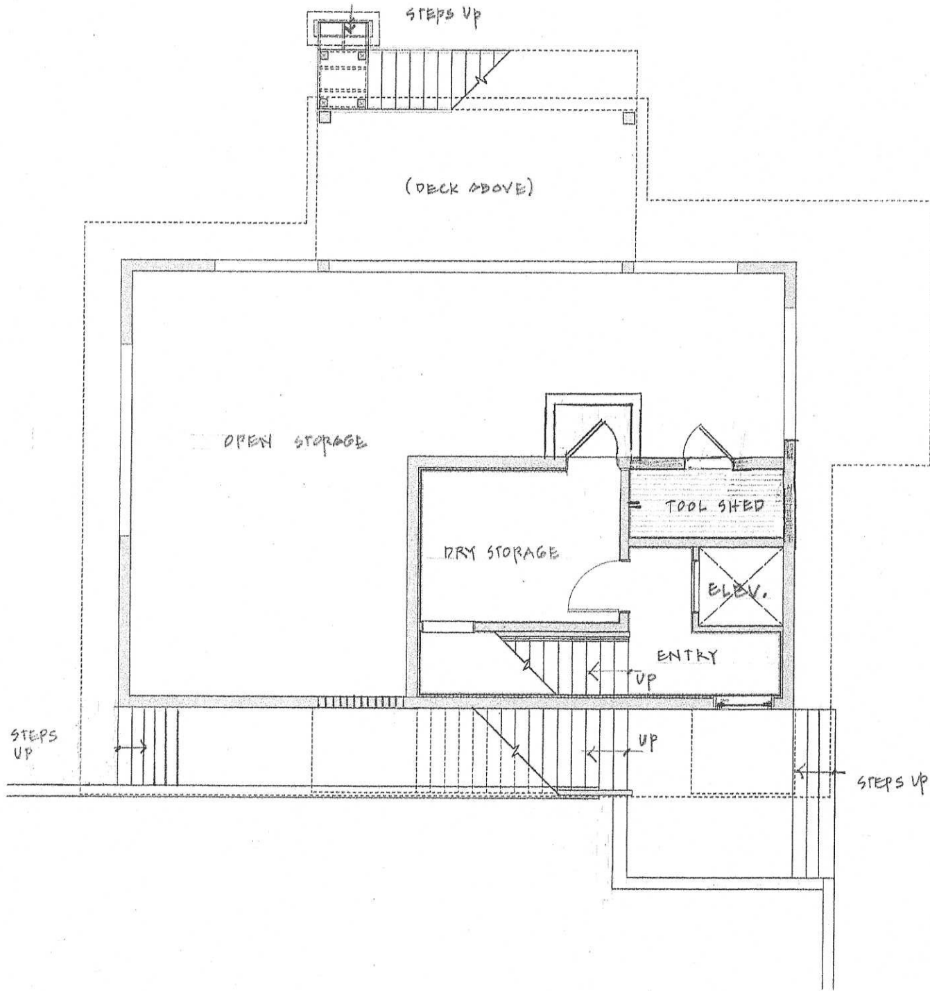
1 GROUND FLOOR PLAN scale: 1/8"=1'-0"
