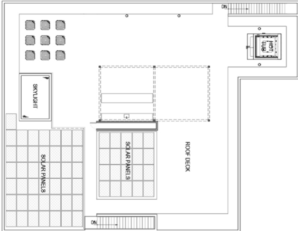
ROOF FLOOR PLAN
